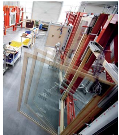
20,000 tilt cycles and up to 30,000 turn cycles: the most important NT components are tested beyond the current standards and guidelines.
