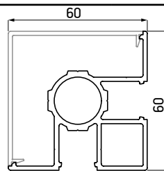
F60 stub skretnica 90° 60×60 mm - 6 m Antracit RAL 7016
