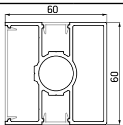
F60 stub 60×60 mm - 6 m Antracit RAL 7016
