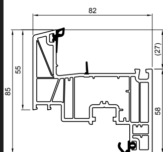
Krilo 82 mm - Antracit
