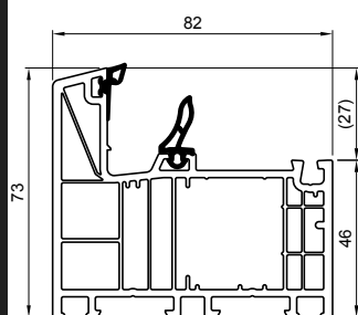
Štok 82 mm MD - Antracit spolja
