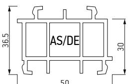
Podštok AS/DE 6 m (LB.Profile 70 mm, Profine 76, Aluplast, Schüco, Alphcan, Profilink, Reiner, Hammer Decco 70/80) PMSLB.AS.DE 9.80€
