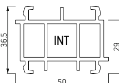
Podštok INT 6 m (Inoutic 70 Arkada, 76 Prestige) PMSLB.INT 9.80€
